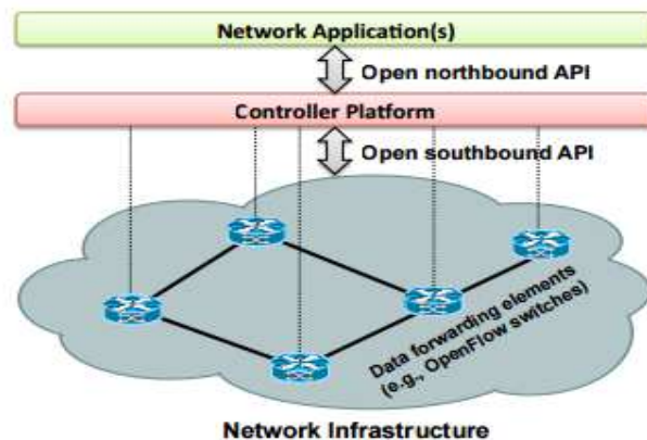
Fig. 1. Simplified view of an SDN architecture.
