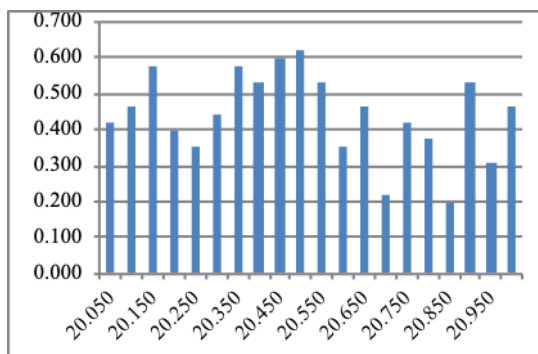
Figure 3. Comparative graph of rebound deflections (mm) with chainages using BBD technique
