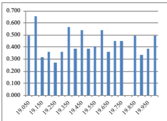
Figure 2. Comparative graph of rebound deflections (mm) with changes(km) using BBD method
