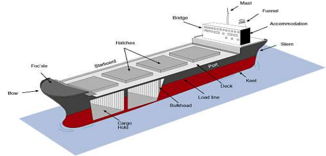
Figure 9: Cargo ship
