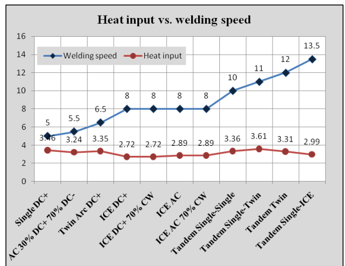
Figure 6. Heat input vs. welding speed
