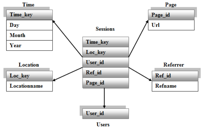
Figure4. Representation of Star schema
